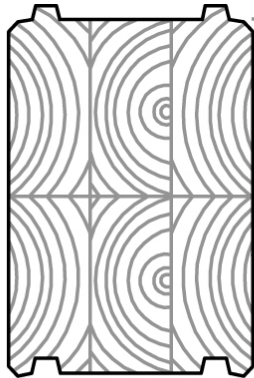
LHV 180x260
